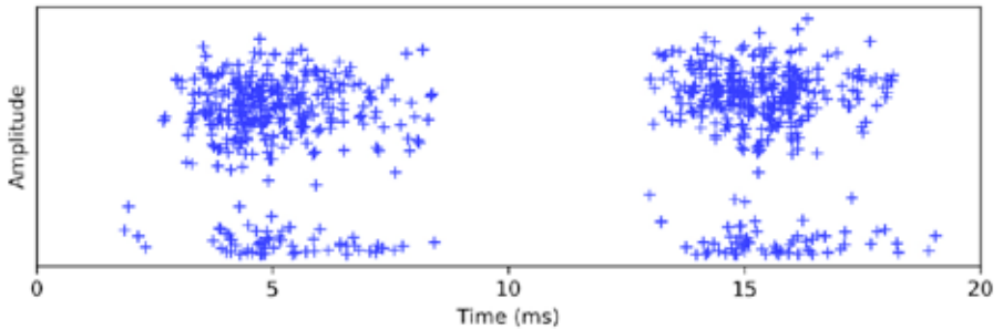
Example of the PRPD pattern of an internal discharge.
