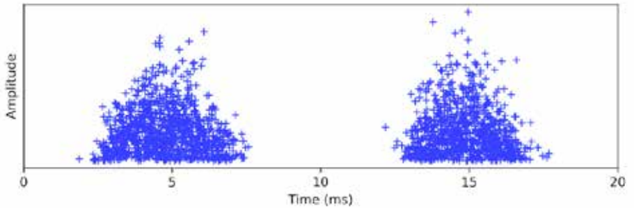
Example of the PRPD pattern of a surface discharge.
