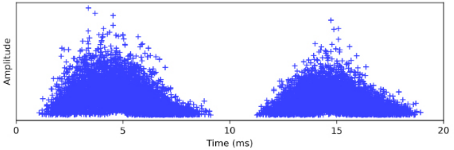
PRPD pattern without reference to the absolute phase of the voltage.
